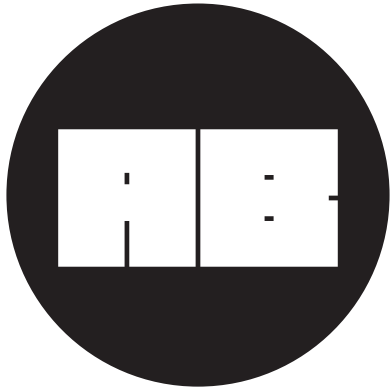
BLACK HOLE
